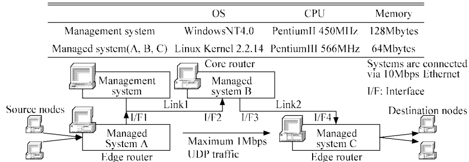
Fig. 11: Network configuration in evaluations.
