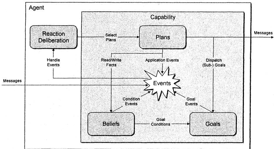
Fig. 1 Jadex architecture
