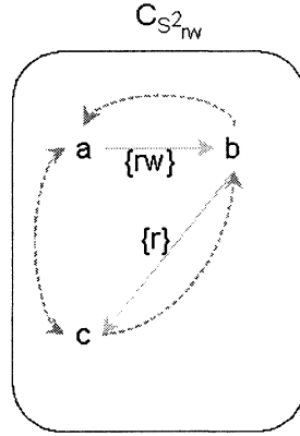
Figure 3. The secure reconfiguration of C_{S_{rw}^1} as C_{S_{rw}^2} (Example 4).
