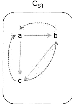
Figure 1. An access flow permitted through transitivity (Example 2).
