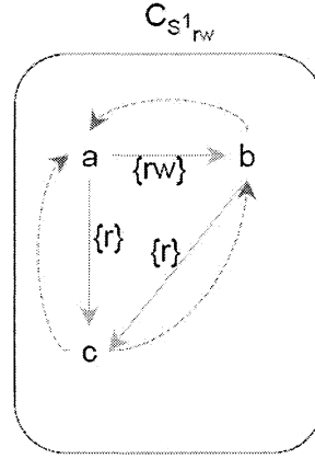
Figure 2. The access flows in the system described in Example 3.
