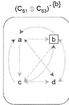
Figure 6. Reconfiguration (\mathcal{C}_{S1} \otimes \mathcal{C}_{S3})^{*\{b\}} (Example 9).
