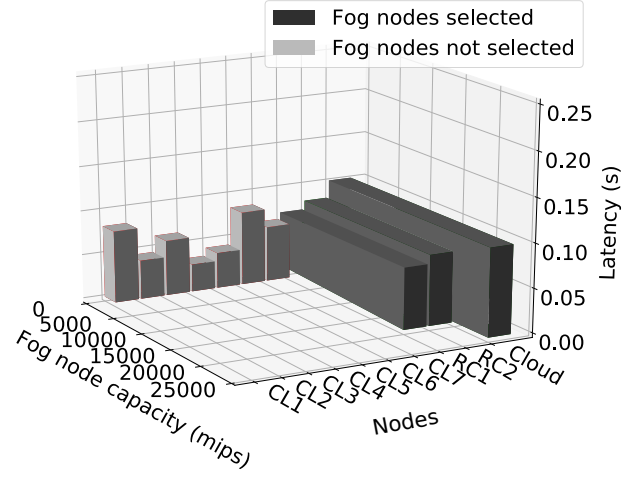
(b) Nodes' hardware capacity and latency
