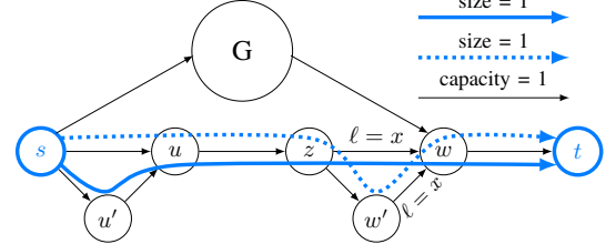
Fig. 6. In this network, the task is to migrate in an latency-consistent way from the flow F , depicted in solid blue, to the flow F' , depicted as a blue dashed path. All edges have a capacity of 1 and a latency of 1, except for (z, w) and (w', w) with a latency of x . The only way to migrate in an latency-consistent fashion is if there is a path P via G from s to w that has a length of exactly x + 3 . Then, one can latency-consistently migrate F to P, w, t , then to F' .
