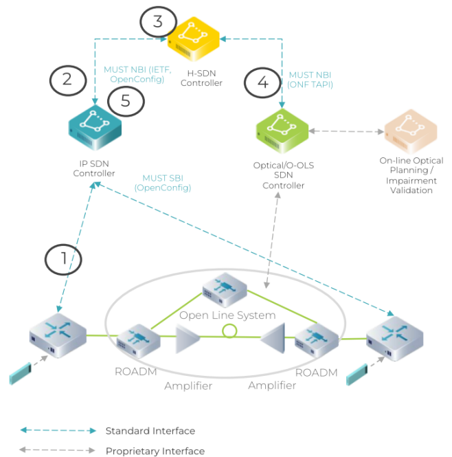
Fig. 1. MANTRA Single SBI management of IPoWDM routers [7], [8]
