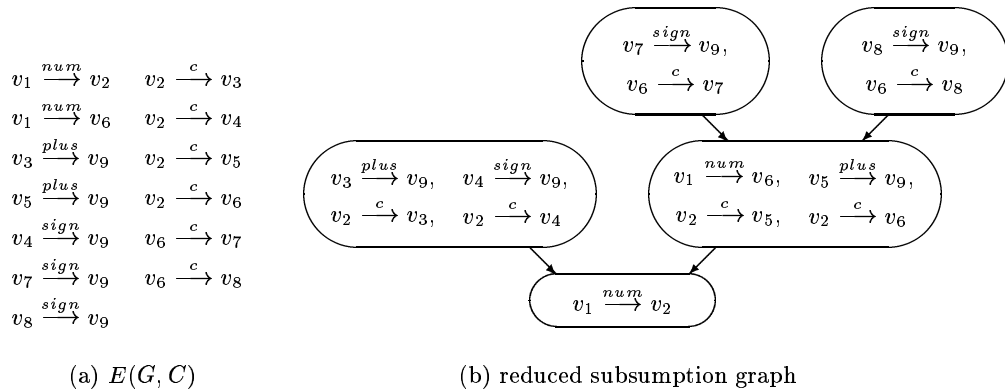
Fig. 5. The reduced subsumption graph for Figure 1 and all-dependence-pairs coverage criterion
