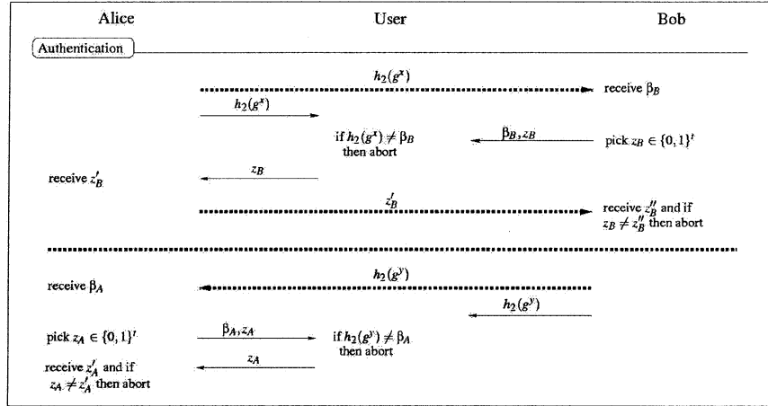
Figure 10. Authentication step in Figure 3 for \text{UAKE}(A \xleftrightarrow[0]{AC} U \xleftrightarrow[0]{AC} B)
