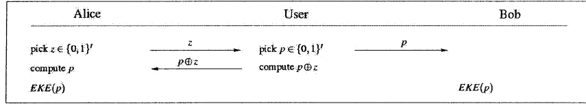
Figure 5. UAKE(A \xleftrightarrow{C} U \xrightarrow{AC} B)
