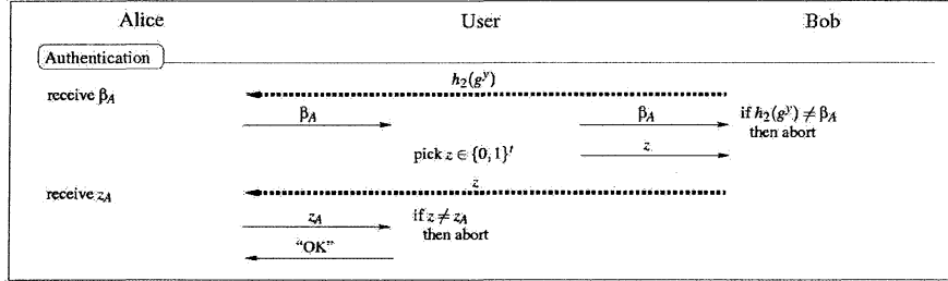
Figure 8. Authenticated channel from Bob to Alice in A \xrightarrow[A]{A} U \xrightarrow[A]{AC} B
