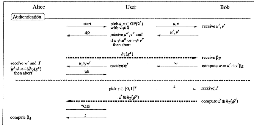
Figure 12. Authenticated step in Figure 3 for \text{UAKE}(A \xleftrightarrow[A]{A} U \xleftrightarrow[C]{C} B)
