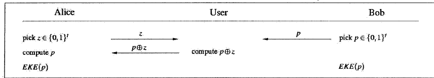
Figure 6. UAKE(A \xleftrightarrow{C} U \xleftarrow{AC} B)
