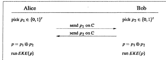
Figure 2. \Phi KE(A \xleftrightarrow[C]{C} B)
