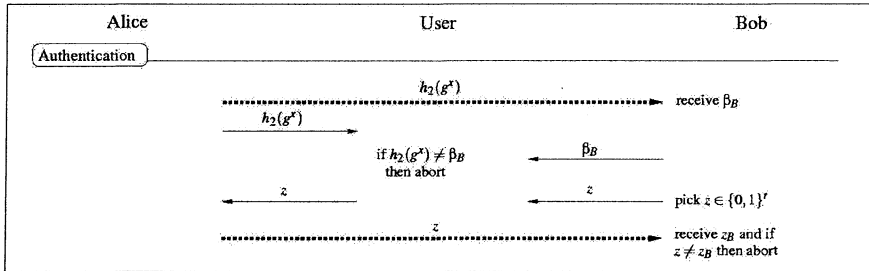
Figure 9. Authenticated channel from Alice to Bob in A \xrightarrow[A]{A} U \xleftarrow[A]{AC} B
