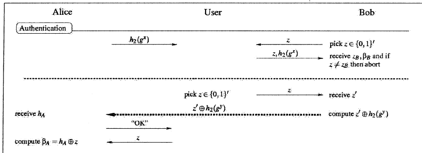
Figure 7. Authentication step in Figure 3 for UAKE(A \xleftrightarrow{A} U \xleftrightarrow{IC} B)
