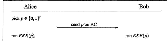
Figure 1. \Phi KE(A \xleftrightarrow[AC]{A} B)
