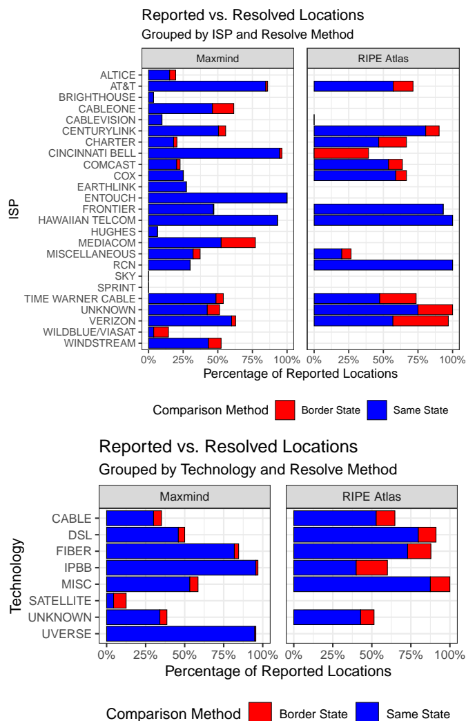
Fig. 4. Reported vs. resolved geographic locations, grouped by resolve method and technology/ISP. To do this, we: (1) for each traceroute take the first public IP, (2) geolocate the US State using that IP using the RIPE method, (3) if the RIPE method does not work, then we use the MaxMind GeoIP mapping as a fallback, (4) take the closest resolved location timestamp to the unit’s reported metadata timestamp.
