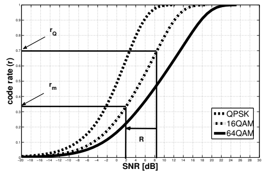
Fig. 2. Normalized BICM Mutual Information and calculation of Shift with respect to the mother code rate
