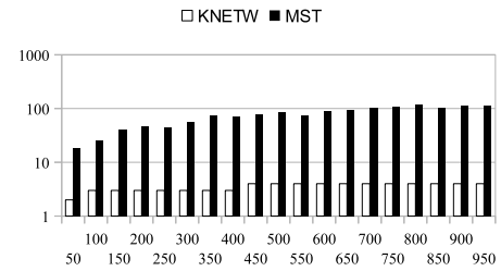
Fig. 7. Max hop-distance from every sensor to the root, H(\cdot) .
