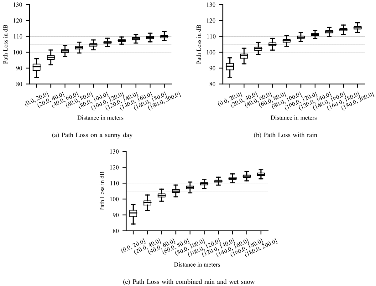
Figure 5. Total path loss results for a rain intensity of 30 mm/h. The horizontal lines indicate a path loss of 100, 105 and 110 dB, respectively
