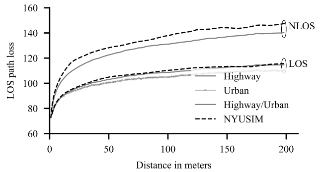
Figure 1. Path loss with increasing Tx-Rx distance at 60 GHz.
