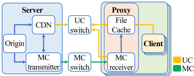
Fig. 1. The system architecture [5]. Multicast is used for emulating a broadcast network.
