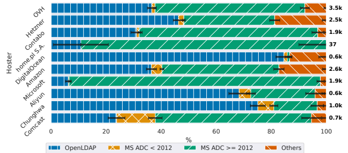
Fig. 2. Most common hosters vs. hosted LDAP products with confidence interval of 95% (horizontal dark bars).
