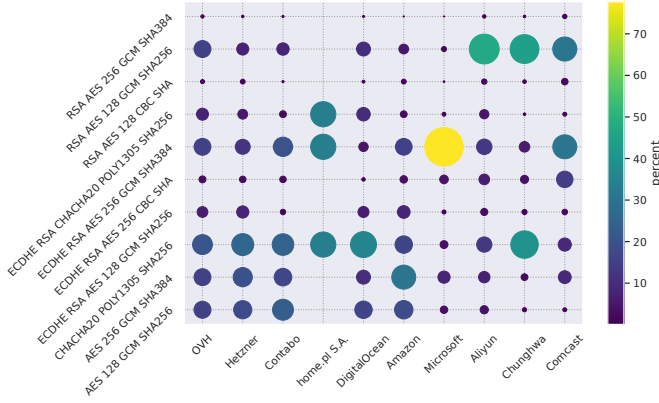
Fig. 3. Percentage of the top 10 cipher suites negotiated with servers on important hosters. The last three entries are TLSv1.3 and use ECDHE for key exchange. These ciphers cover 98% of what servers selected in our data.
