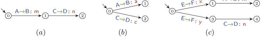
Fig. 3. Well-formedness is necessary for Theorem 4.14.
