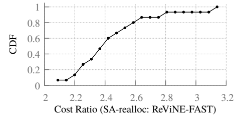
Fig. 5. Large inputs run for \leq 5 minute
