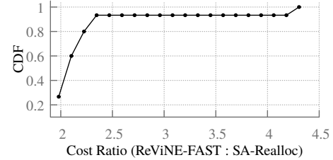
(b) Cost Ratio of SA-realloc [7] to ReViNE-FAST
