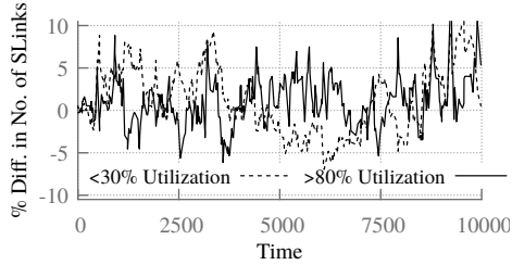
(b) Impact on Load Distribution
