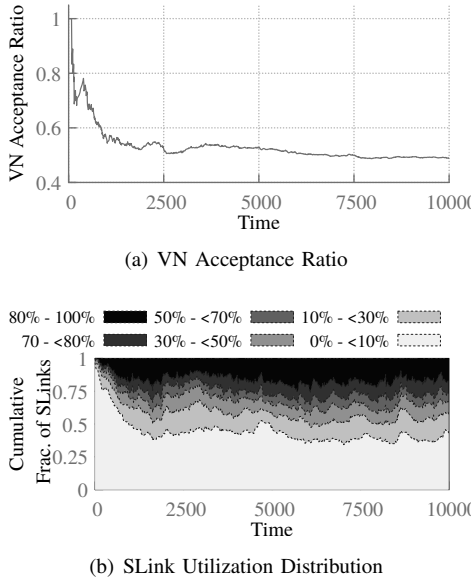
Fig. 1. Results for Motivating Example
