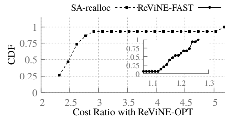
(a) Cost Ratio Comparison
