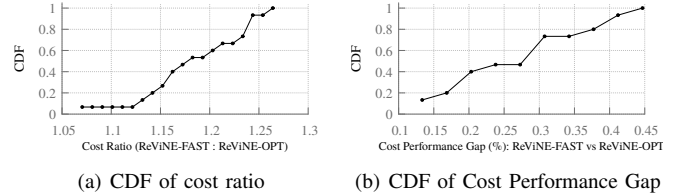
Fig. 2. Comparison between ReViNE-OPT and ReViNE-FAST
