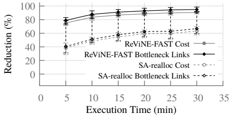
Fig. 6. Convergence behavior comparison
