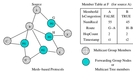
Fig. 1. Member table maintained for local recovery
