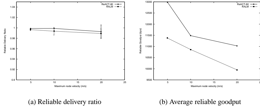
Fig. 3. Effect of mobility
