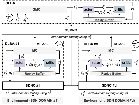
Fig. 2. Data exchange between the domain and global level entities (i.e., b_{ij}, c_{ij}, u_{ij}, b_m ) and calculates \Gamma^d and \varphi^d . The DLBA's actor consumes s_t^d to provide domain routing graph a_t^d . MC also derives the abstracted domain graph to obtain the abstracted domain load balancing factor \varphi^{da} for DLBA reward calculation. The abstracted domain graph is extended by the visible inter-domain links (with associated parameters) to obtain abstracted domain state s_t^{da} provided to Global Metrics Calculator (GMC). GMC joins the s_t^{da} received from each domain (eliminating link duplication) to get a global network state s_t^g , which is used to obtain rewards and global routing graph a_t^g , as in DLBA case. The routing graphs are sent to relevant SDNCs/GSDNC to be used for Dijkstra-based routing until the next update by DLBA/GLBA. Due to SDN specifics, to reduce SDNC load, the policy is updated every time interval T^x ( T^d for DLBA, T^g for GLBA, T^g \gg T^d ), equal to the state sampling frequency. Each domain can, therefore, operate at a different time scale, as the network flows are routed using the current domains' routing graphs.
