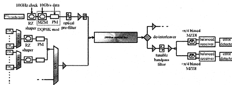
Figure 1. Experimental setup.
