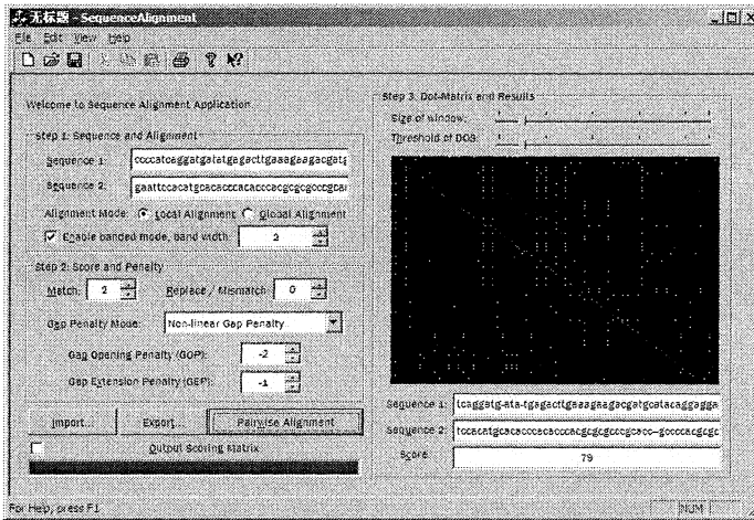
Figure 3. Visualized implementation of sequence alignment algorithms
