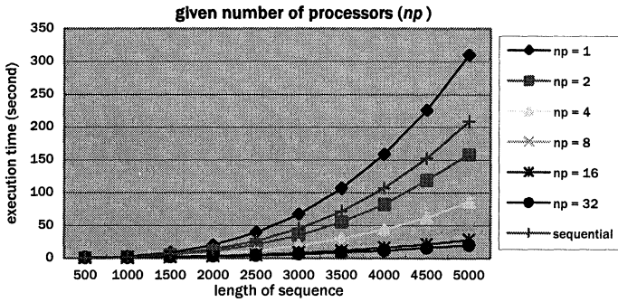
Figure 9. Execution time for various lengths of sequence
