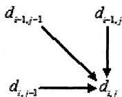
Figure 4. Data dependency in computing elements of score matrix
