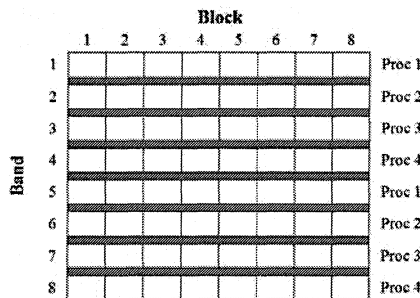
Figure 8. A 8*8 partition for 4 processors
