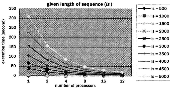
Figure 10. Execution time for various numbers of processors
