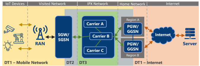
Figure 1: Roaming network infrastructure and data sources.
