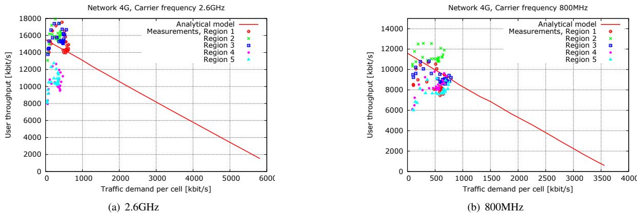
Fig. 4. Mean user throughput versus traffic demand for 4G in Country 1 at two different frequency bandwidths.
