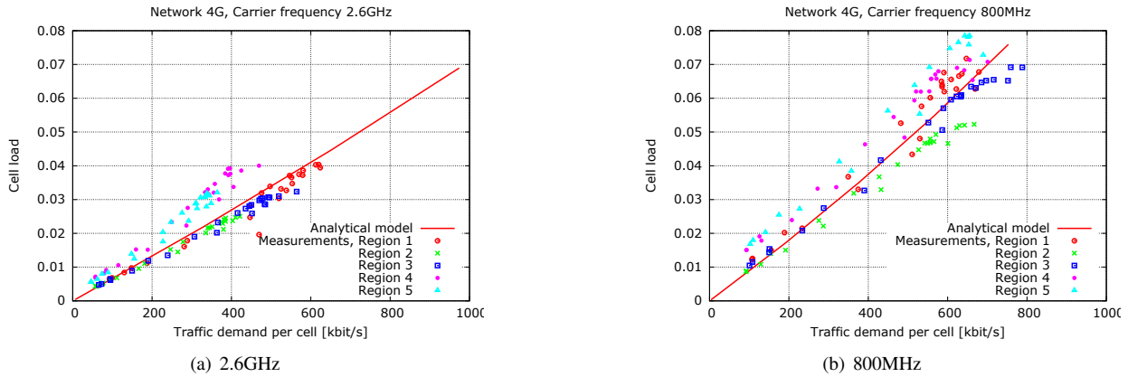
Fig. 3. Mean cell load versus traffic demand for 4G in Country 1 at two different frequency bandwidths.
