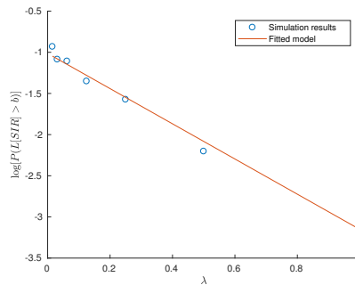
Fig. 3: Simulation estimate of \log \mathbb{P}(L_\lambda[\text{SIR}] > b) with \tau = -50 dB and \epsilon = 0.01 , fitted to a linear model \hat{y}_1 = p_1\lambda + p_2 , where p_1 = -2.138 and p_2 = -1.014 . The value of -p_1 is an estimate for the rate function.
