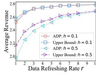
Fig. 1. The average revenue under the approximate dynamic pricing policy with data refreshing rate r .
