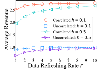
Fig. 2. The value of data correlation under dynamic pricing policy with data refreshing rate r .
