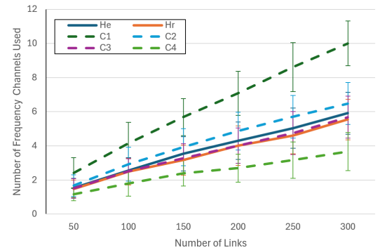
Fig. 8: Average frequency usage to deconflict 100 random topologies with up to 300 dir-dir links using different directional SCMs.
