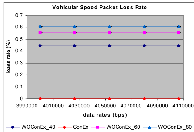
Fig 7. Walking Speed Packet Loss Rates Analysis
