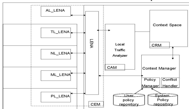
Fig 1. CA3Rm-Com Architecture.
