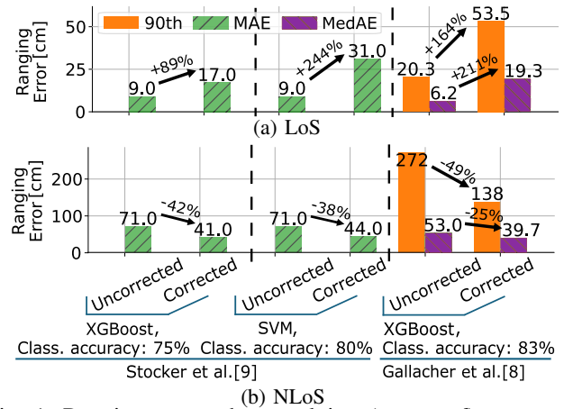
Fig. 1: Ranging error when applying ( corrected ) or not applying ( uncorrected ) SoA ranging correction methods [8], [9]. The correction is clearly effective in NLoS conditions (b), but has a negative impact on ranging estimates taken in LoS (a). 90^{th} : 90^{th} percentile of the absolute ranging error; MAE : mean absolute error; MedAE : median absolute error.
