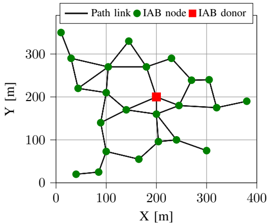
Fig. 1: Simulation Scenario
