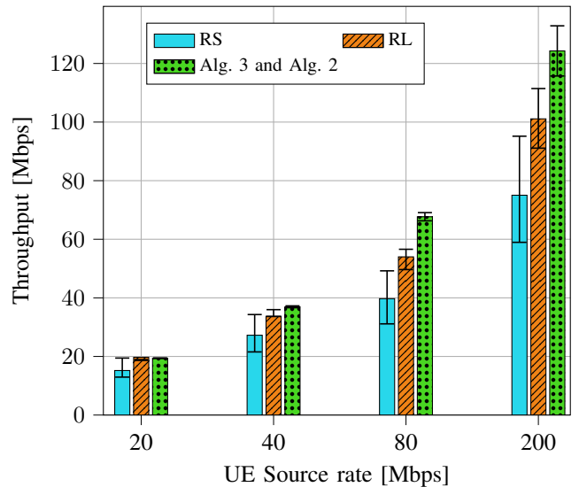
Fig. 2: Throughput per UE for different schedulers and THz link selection policies, for THz bandwidth 32 GHz and \rho_{max} = 0.3 .
